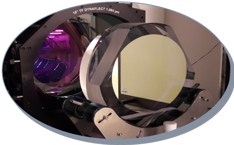
Miroir VIRGO
